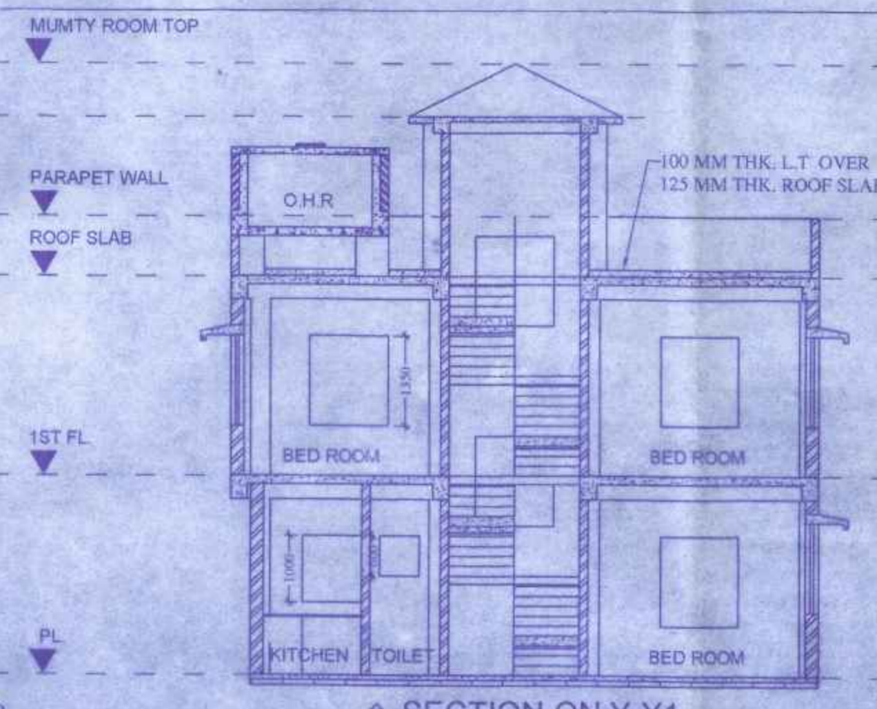
SECTION ON Y-Y1 SCALE :- 1:100
