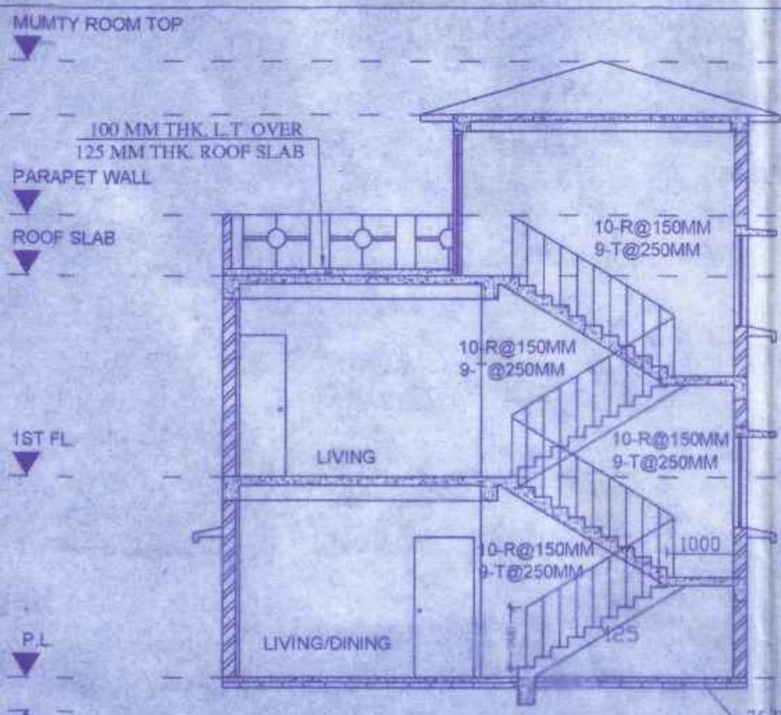
SECTION ON X-X1 SCALE :- 1:100
